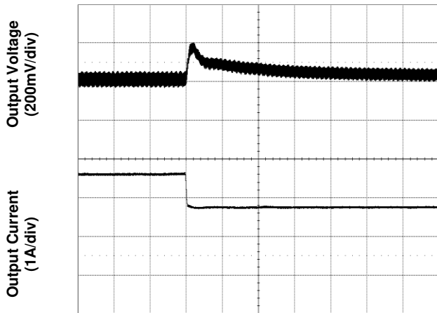
Time – t (100µs/div) Figure 7. Transient Load Response (typical Vin, load current steps from 75% to 50% at a slew rate 0.1A/µs)
