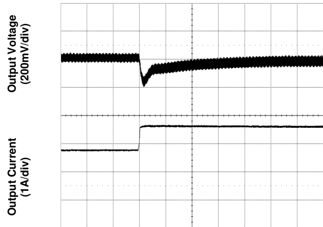
Time – t (100µs/div) Figure 8. Transient Load Response (typical Vin, load current steps from 50% to 75% at a slew rate 0.1A/µs)
