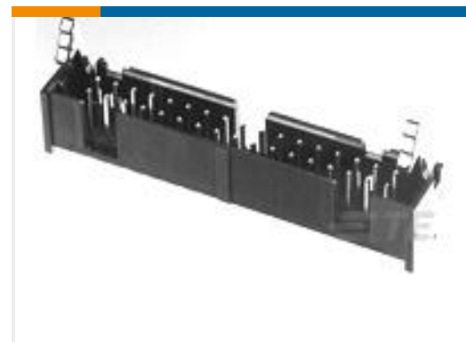
TE Part #1-1761606-5 IDC LOW PRO HDR 50P VERT LG LA
