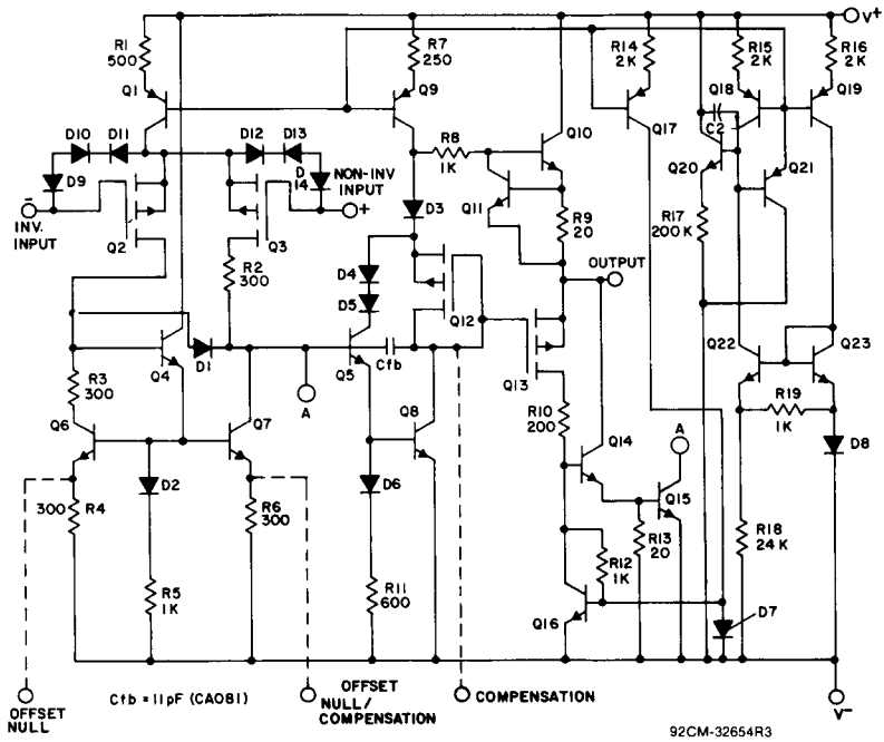
Fig. 1 - Schematic diagram of the CA081, CA082, and CA084.
