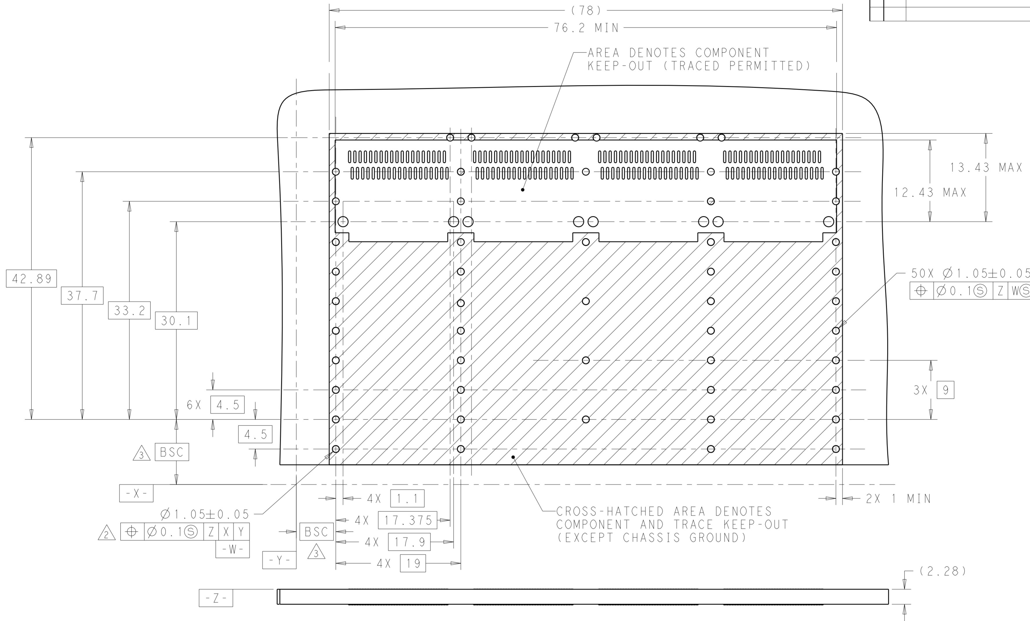
RECOMMENDED PCB LAYOUT BELLY TO BELLY MOUNTED CONFIGURATION SCALE 3:1
