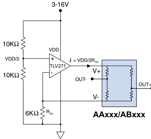
Figure 11. Constant-current supply.
