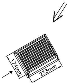
Blister box bottom
