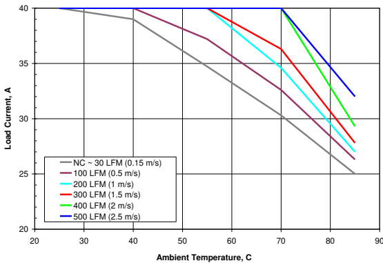
Figure 1. Available load current vs. ambient air temperature and airflow rates for SQE48T40015 converter mounted vertically with air flowing from pin 3 to pin 1, MOSFET temperature \leq 120^\circ\text{C} , V_{in} = 48\text{ V} . Note: NC – Natural convection
