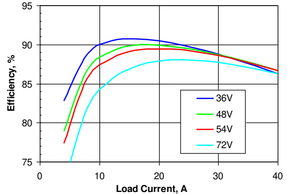
Figure 2. Efficiency vs. load current and input voltage for SQE48T40015 converter mounted vertically with air flowing from pin 3 to pin 1 at 300 LFM (1.5 m/s) and T_a=25^\circ\text{C} .
