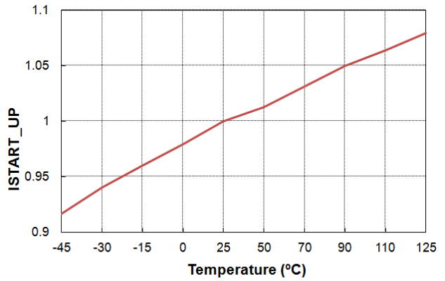
Figure 12. ISTARTUP vs. Temperature
