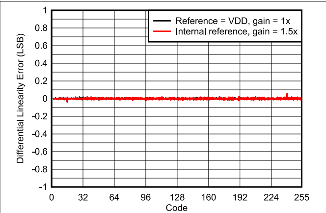
Figure 6-2. Differential Linearity Error vs Digital Input Code
