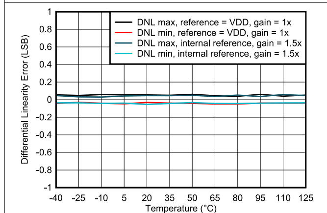
Figure 6-5. Differential Linearity Error vs Temperature
