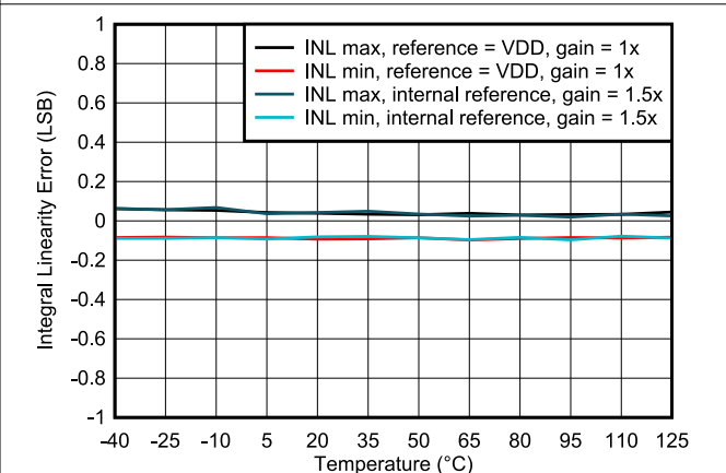
Figure 6-4. Integral Linearity Error vs Temperature
