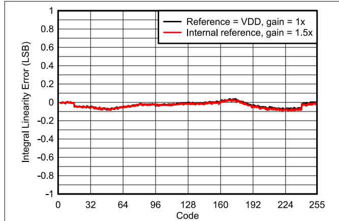
Figure 6-1. Integral Linearity Error vs Digital Input Code
