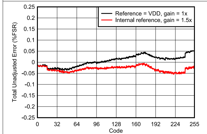
Figure 6-3. Total Unadjusted Error vs Digital Input Code
