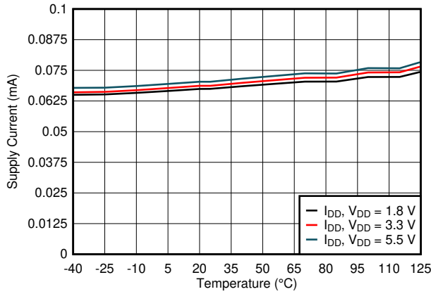
Figure 6-33. Power-Down Current vs Temperature
