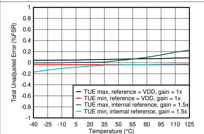
Figure 6-6. Total Unadjusted Error vs Temperature
