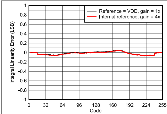
Figure 6-11. Integral Linearity Error vs Digital Input Code
