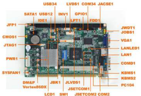
Jumper and Connector Locations (component side)
