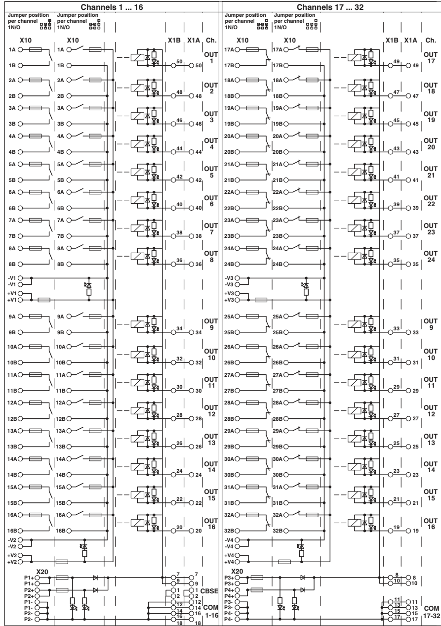
Circuit diagram
