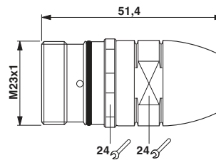
Dimensioned drawing
