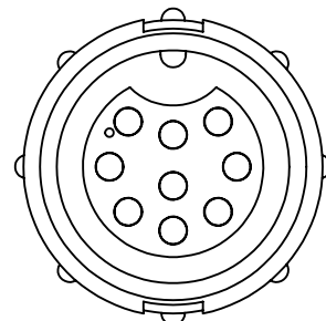
W5282-9SG-P-3XX MATING VIEW
