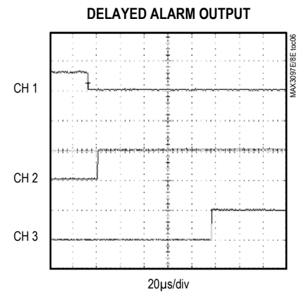
CH1: V_A , 5V/div CH2: V_{ALARMA} , 5V/div CH3: V_{ALARM} , 5V/div V_A = GND , C_{DELAY} = 270pF
