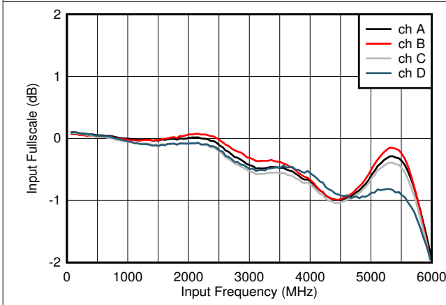
Figure 7-3. Input Fullscale vs Input Frequency
