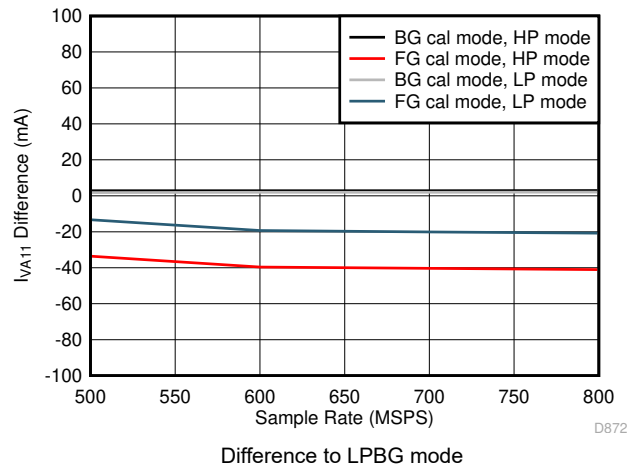
Figure 7-100. Dual Channel, I_{VA11} vs F_S over Modes
