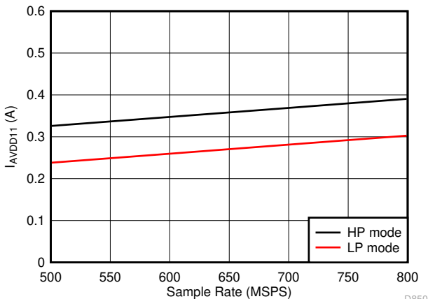
Independent of JMODE Figure 7-93. Dual Channel, I_{VA11} vs F_S
