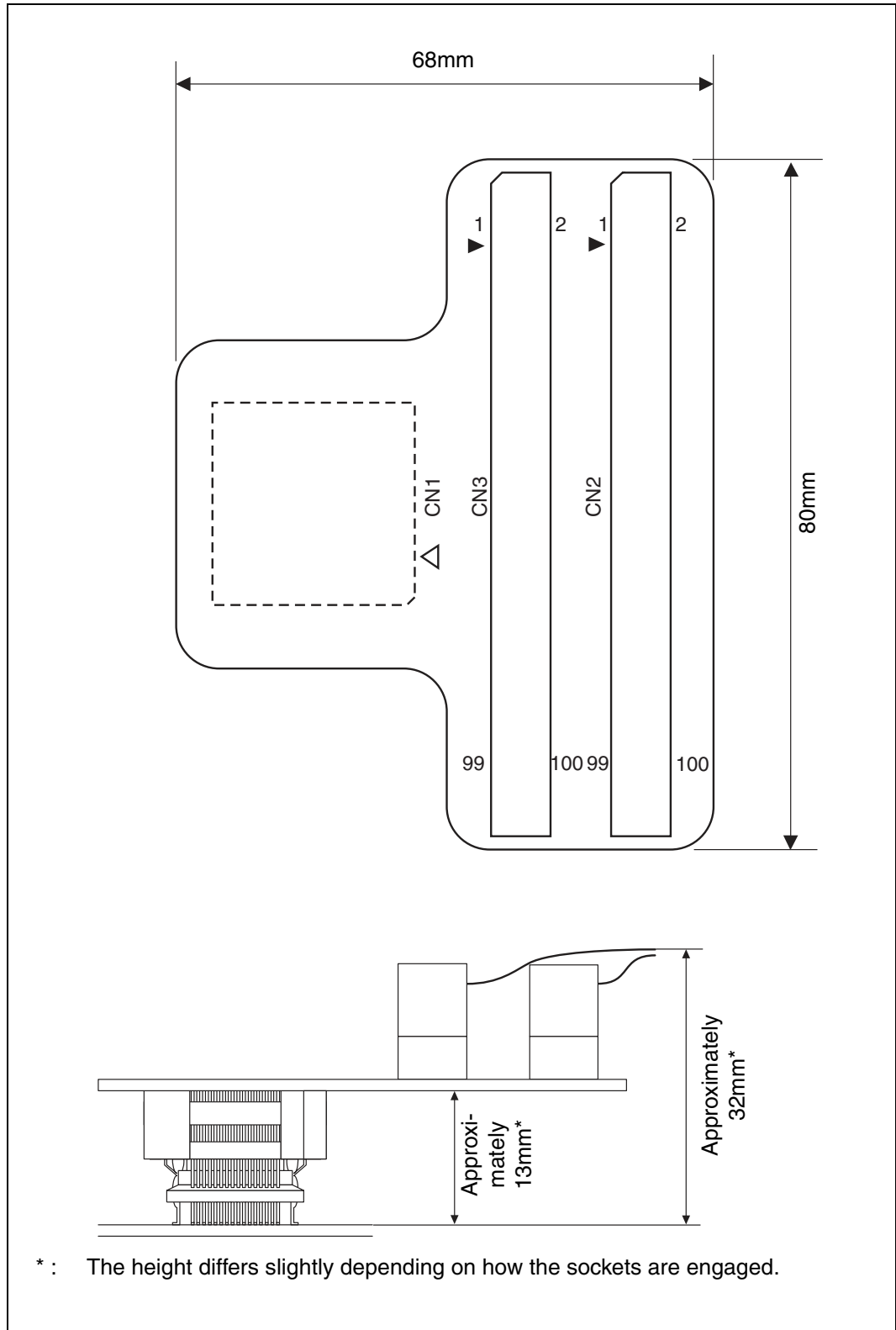
Figure 1 Header board dimensions
