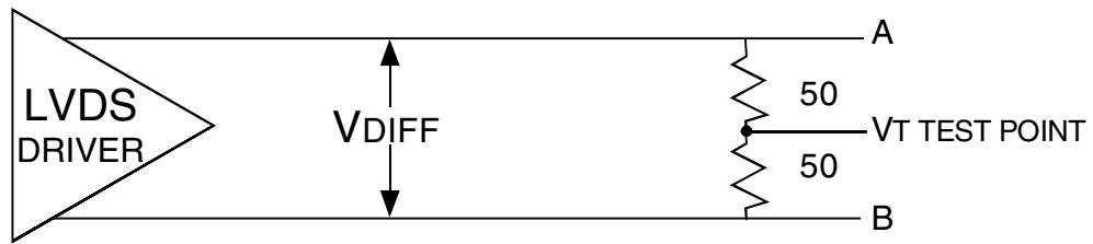
Test Circuit for LVDS Output Characteristics
