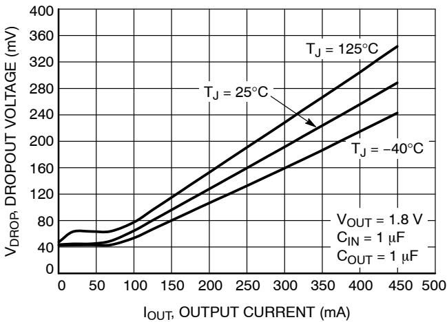
Figure 18. Dropout Voltage vs. Load Current – V OUT = 1.8 V
