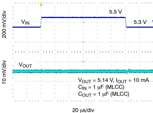
Figure 41. Line Transient Response – V_{OUT} = 5.14\text{ V}
