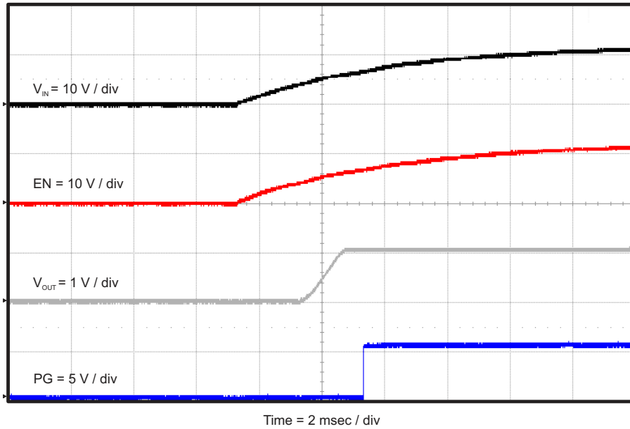
Figure 4-11. TPS54625EVM-608 Start-Up Relative to V_{IN}
