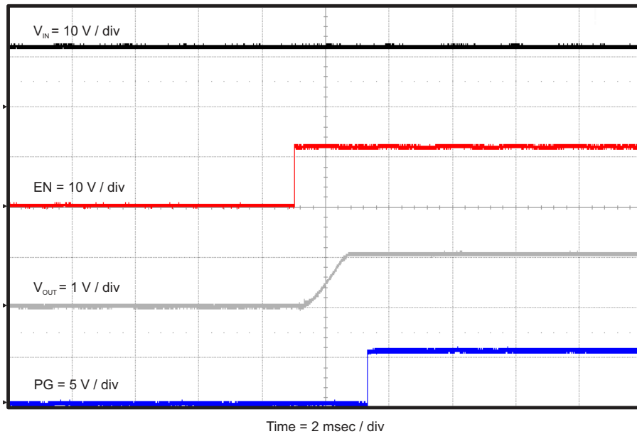
Figure 4-12. TPS54625EVM-608 Start-Up Relative to EN
