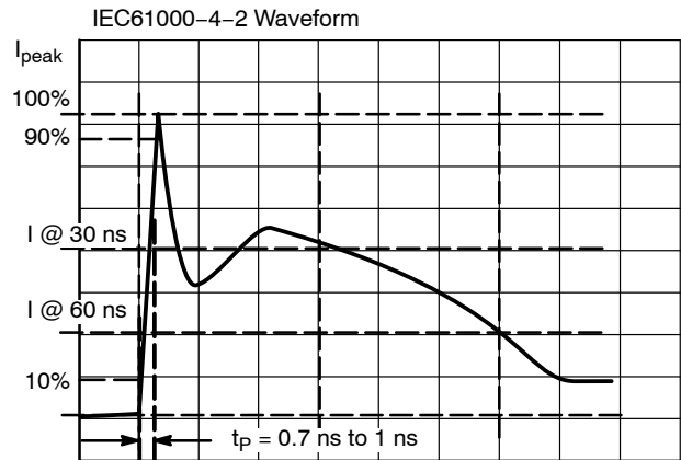
Figure 12. IEC61000-4-2 Spec
