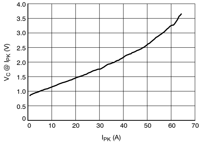
Figure 5. Negative Clamping Voltage vs. Peak Pulse Current ( t_p = 8/20 \mu s)
