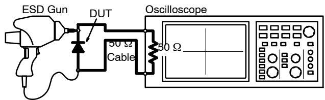
Figure 13. Diagram of ESD Test Setup
