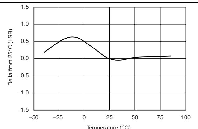
Figure 7. Change in Offset vs Temperature
