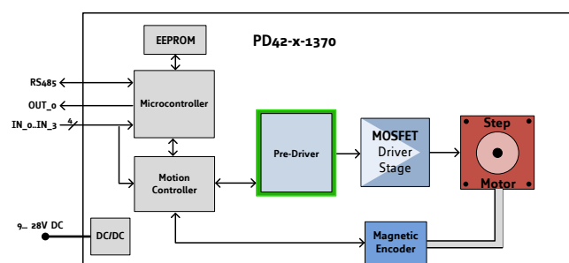
Figure 13: PD42-x-1370 block diagram
