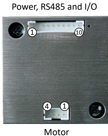
Figure 2: PD42-x-1370 connectors
