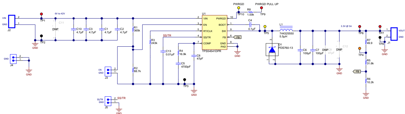
Figure 2. TPS54541EVM-555 Schematic
