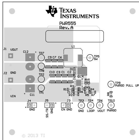
Figure 22. TPS54541EVM-555 Top Assembly and Silkscreen
