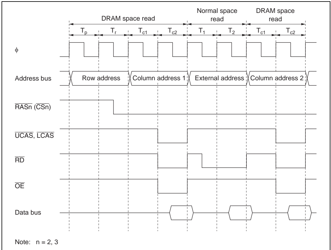
Figure 6.31 Example of Operation Timing in RAS Down Mode (RAST = 0, CAST = 0)
