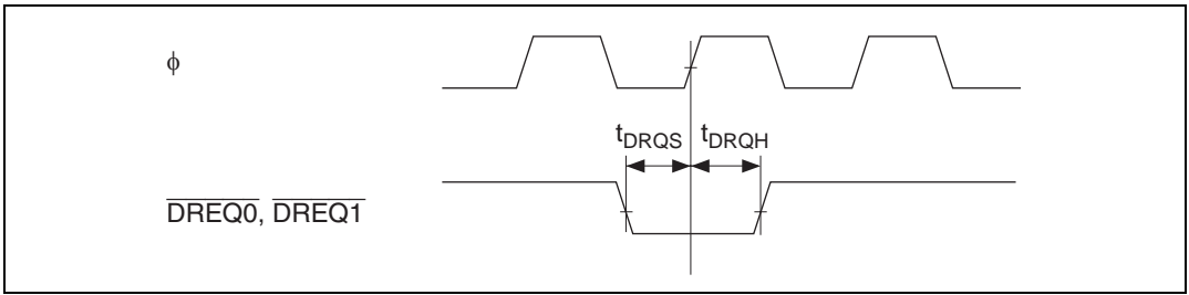
Figure 25.27 DMAC \overline{DREQ} Input Timing
