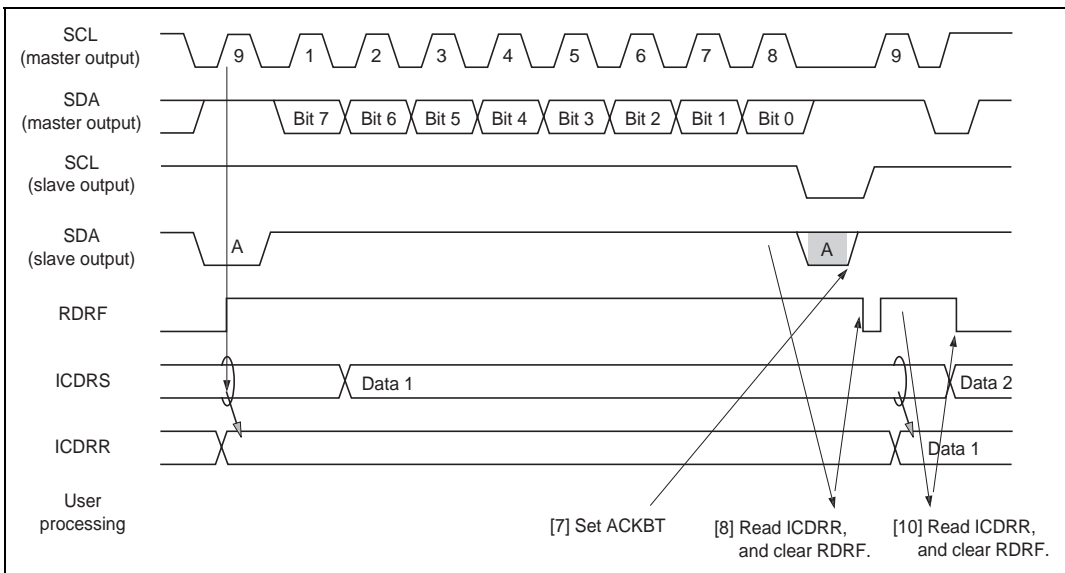
Figure 15.12 Slave Receive Mode Operation Timing 2
