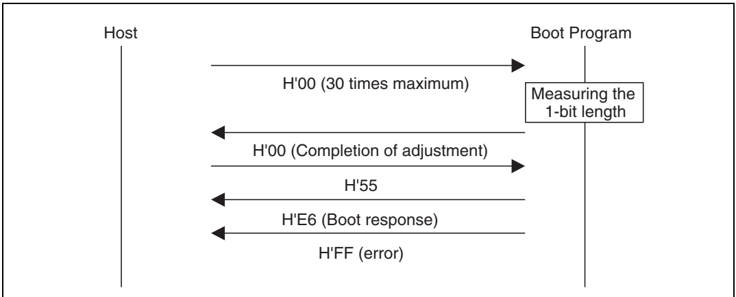
Figure 20.18 Bit-Rate-Adjustment Sequence
