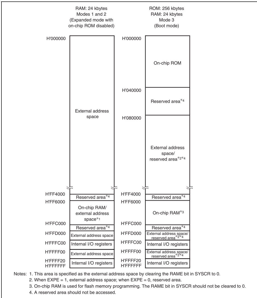
Figure 3.9 H8S/2361F Memory Map (1)
