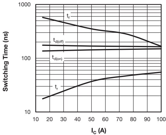
Fig. 12 - Typical IGBT Switching Time vs. I_C T_J = 125\text{ }^\circ\text{C} , V_{CC} = 600\text{ V} , R_g = 2.2\ \Omega , V_{GE} = 15\text{ V} , L = 500\ \mu\text{H}
