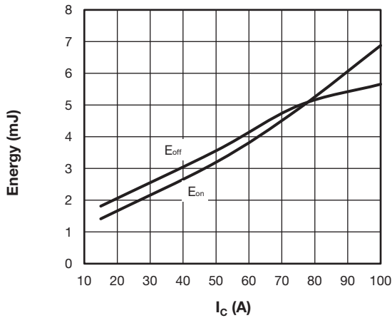
Fig. 11 - Typical IGBT Energy Loss vs. I_C T_J = 125\text{ }^\circ\text{C} , V_{CC} = 600\text{ V} , R_g = 2.2\ \Omega , V_{GE} = 15\text{ V} , L = 500\ \mu\text{H}
