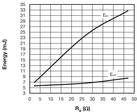
Fig. 13 - Typical IGBT Energy Loss vs. R_g T_J = 125\text{ }^\circ\text{C} , V_{CC} = 600\text{ V} , I_C = 100\text{ A} , V_{GE} = 15\text{ V} , L = 500\ \mu\text{H}
