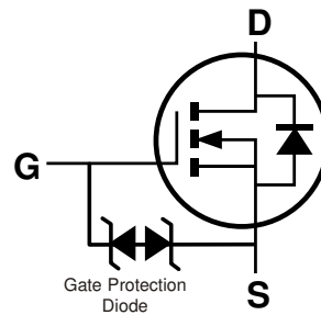
Equivalent Circuit
