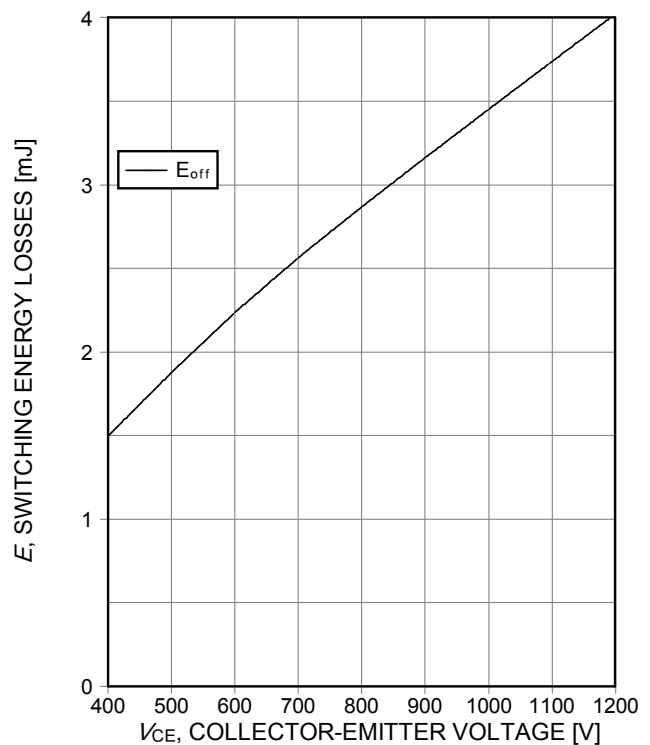
Figure 16. Typical switching energy losses as a function of collector emitter voltage (inductive load, T_{vj}=175^\circ\text{C} , V_{GE}=15/0\text{V} , I_c=20\text{A} , r_G=15\Omega , Dynamic test circuit in Figure E)
