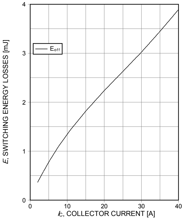
Figure 13. Typical switching energy losses as a function of collector current (inductive load, T_{vj}=175^\circ\text{C} , V_{CE}=600\text{V} , V_{GE}=15/0\text{V} , r_G=15\Omega , Dynamic test circuit in Figure E)
