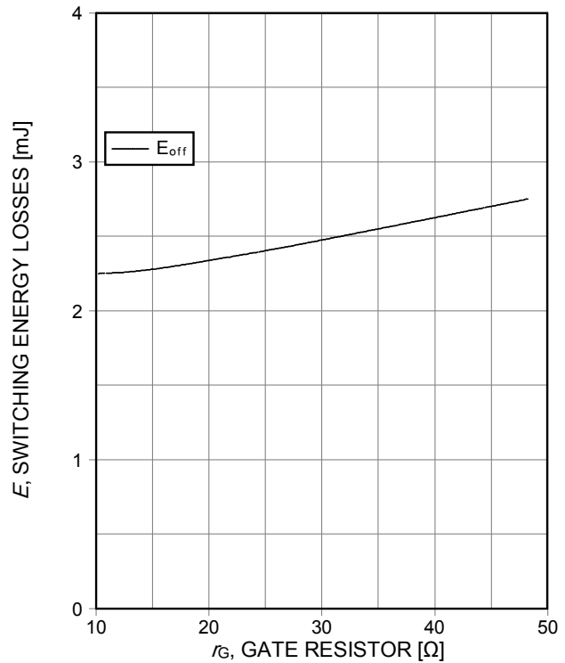
Figure 14. Typical switching energy losses as a function of gate resistor (inductive load, T_{vj}=175^\circ\text{C} , V_{CE}=600\text{V} , V_{GE}=15/0\text{V} , I_c=20\text{A} , Dynamic test circuit in Figure E)
