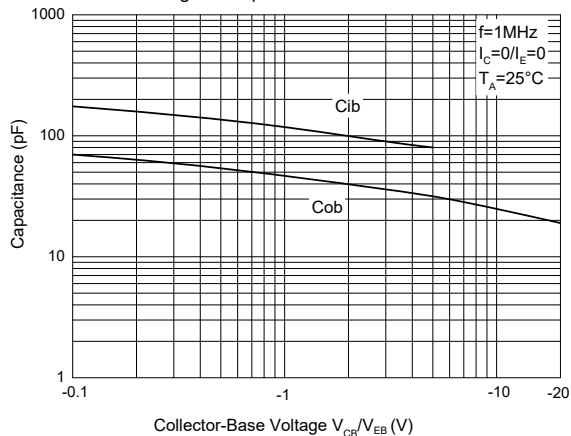
Fig. 5 - Capacitance Characteristics
