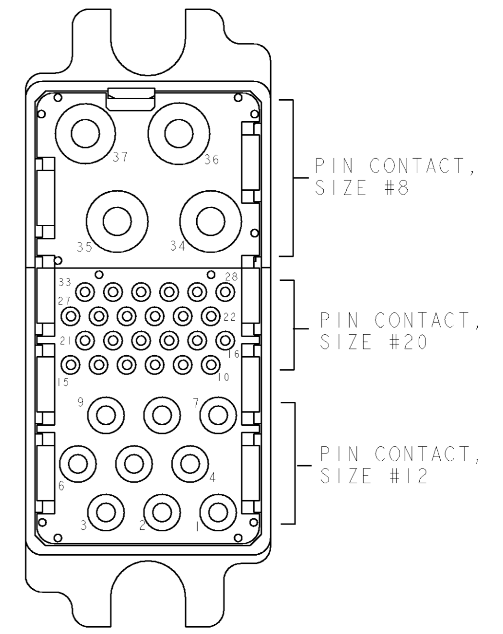
REAR VIEW
