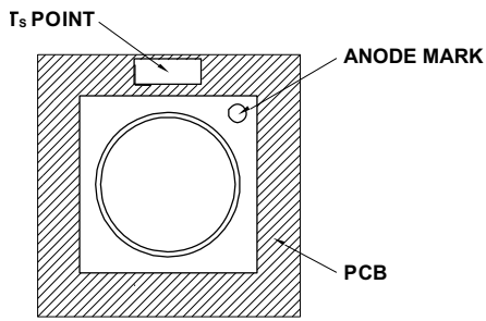
Figure 22: Solder Point Temperature on PCB
