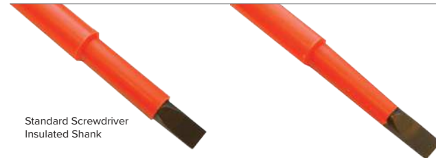
Low Profile Screwdriver Insulated Shaft
