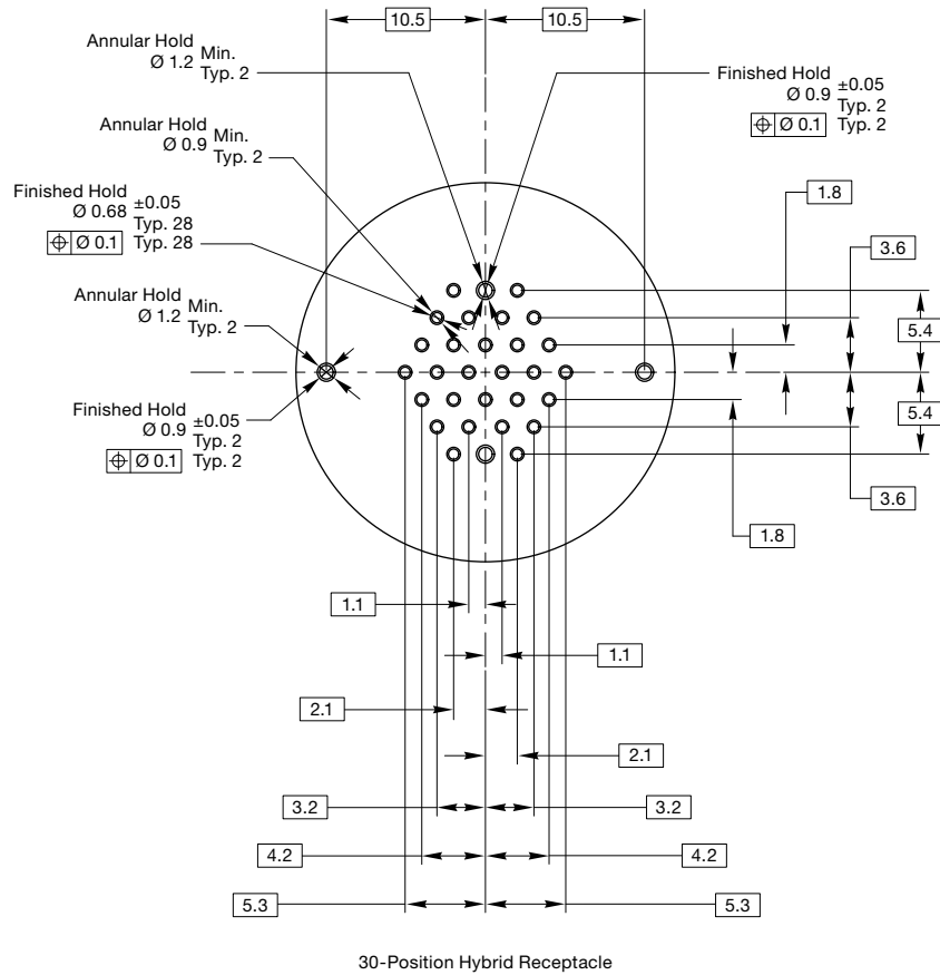
30-Position Hybrid Receptacle
