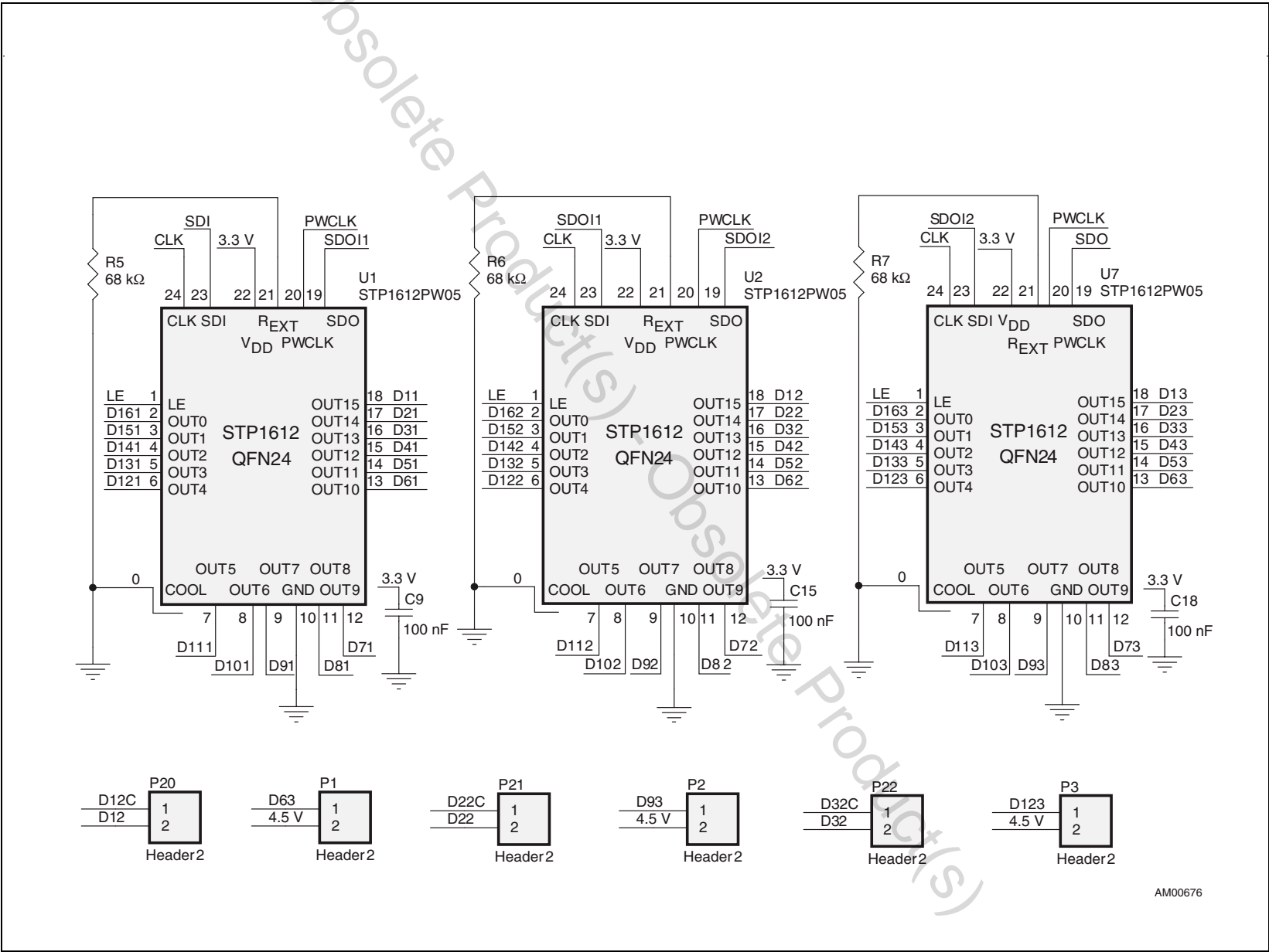
Figure 4. LED drivers
