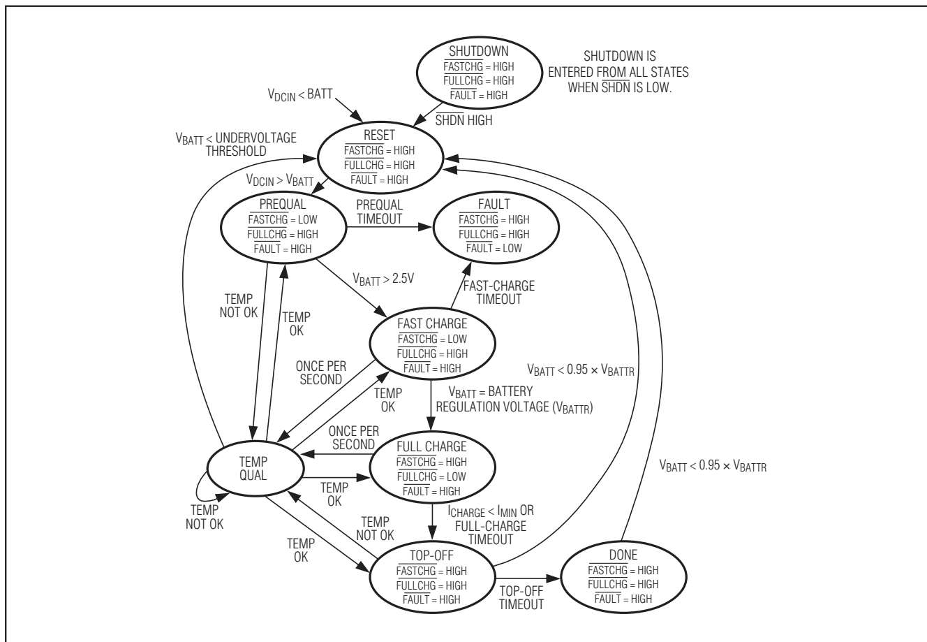
Figure 4. State Diagram
