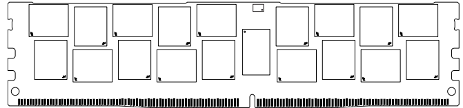
Figure 1: 288-Pin LRDIMM (MO-309, R/C-E)
