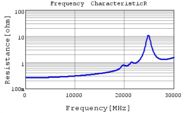
GJM0335C1E1R3CB01 R DC0V,25degC
