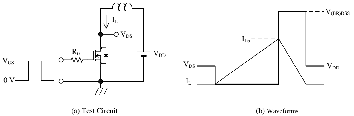
Figure 1 Unclamped Inductive
