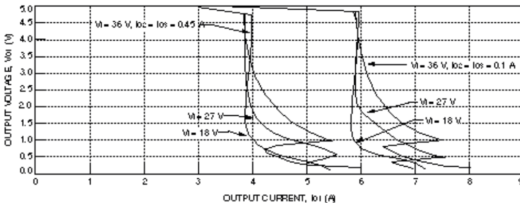
Figure 11. CC025ACL-M Typical 5 V Output Characteristics
