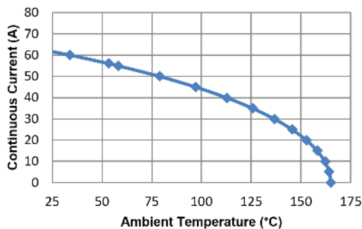
Figure 5: Maximum Continuous Current at a Given T_A
