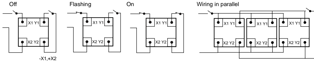
Flashing pilot light base ZB2BV184
