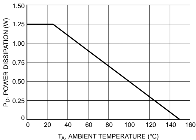
Figure 7. Power Derating
