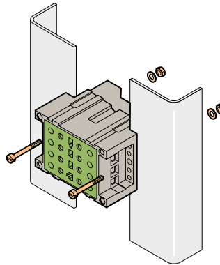
Flush mounting
