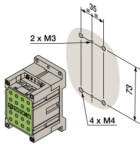
Base mounting
