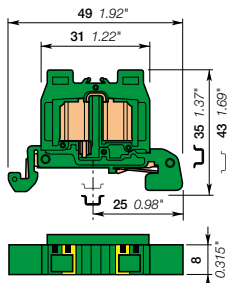
8 mm 0.315 in spacing
