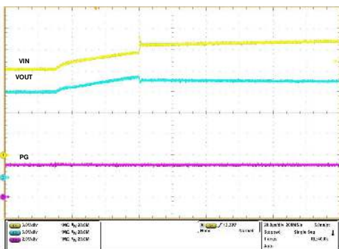
ROVCSSEL = 390 \text{ k}\Omega , C_{OUT} = 220 \mu\text{F} , I_{OUT} = 300 \text{ mA} , V_{IN} ramped up from 12 V to 16.5 V
