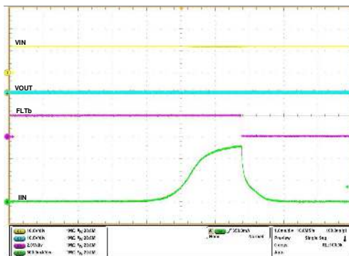
V_{IN} = 12\text{ V} , C_{OUT} = \text{Open} , I_{OUT} short-circuit to GND, R_{ILM} = 1650\text{ }\Omega , V_{EN/UVLO} stepped from 0 V to 3.3 V
