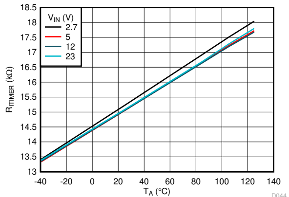
Figure 7-30. ITIMER Internal Pullup Resistance vs Temperature
