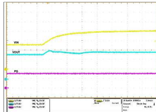
ROVCSSEL = \text{Open} , C_{OUT} = 220 \mu\text{F} , I_{OUT} = 150 \text{ mA} , V_{IN} ramped up from 5 V to 8 V
