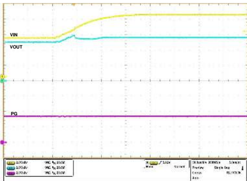
ROVCSSEL = \text{GND} , C_{OUT} = 220 \mu\text{F} , I_{OUT} = 120 \text{ mA} , V_{IN} ramped up from 3.3 V to 6 V
