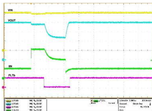
V_{IN} = 12 \text{ V} , C_{TIMER} = 2.2 \text{ nF} , C_{OUT} = 220 \mu\text{F} , R_{ILM} = 549 \Omega , I_{OUT} stepped from 3 A → 9 A → 3 A within 5 ms
