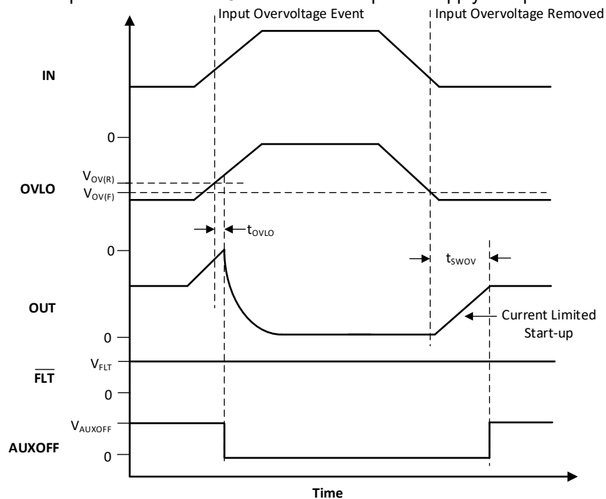
Figure 8-6. TPS259470x Overtolerance Lockout and Recovery
