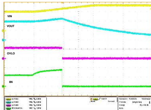
C_{OUT} = 220 \mu\text{F} , R_{OUT} = 20 \Omega , V_{IN} Overvoltage threshold set to 13.2 V, V_{IN} ramped up from 12 V to 16 V
