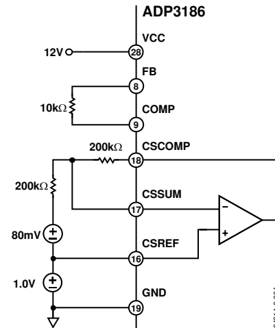
Figure 4. Positioning Voltage
