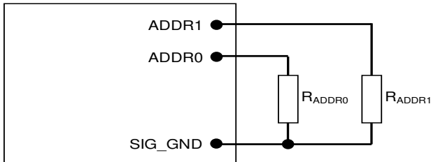
Figure 23. Circuit showing connection of resistors used to set the PMBus address of the module.
