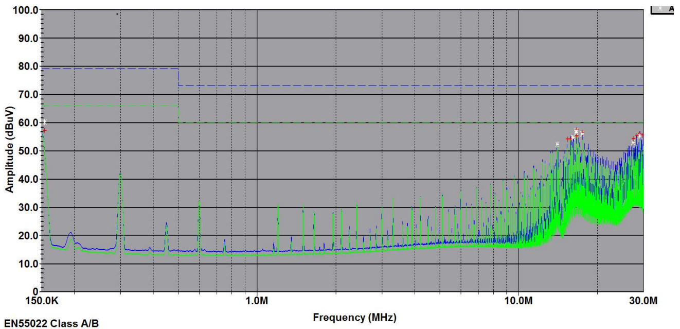
Figure 24. EMC Consideration
