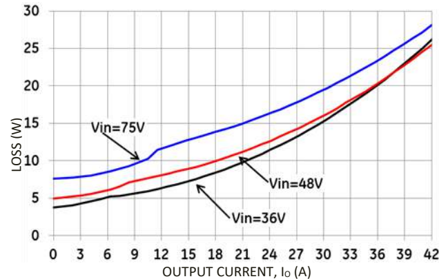
Figure 2. Typical Converter Loss vs. Output Current.
