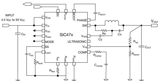
Fig. 1 - Typical Application Circuit for SiC47x
