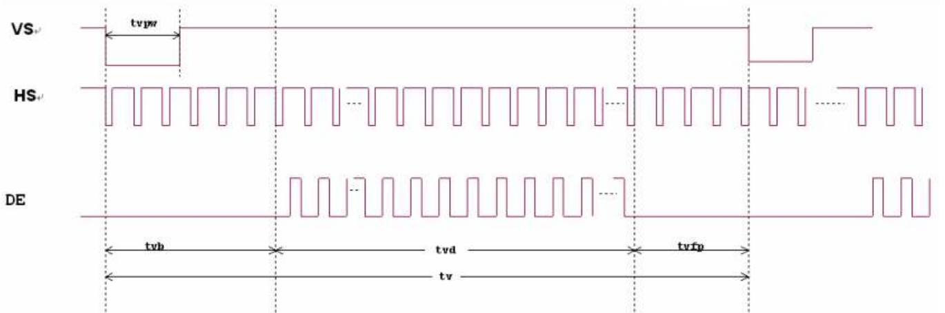
Figure 6: Vertical Input Timing Diagram
