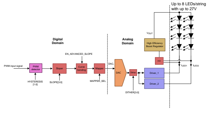
Figure 40. Brightness Control with BRT_MODE bit 01
