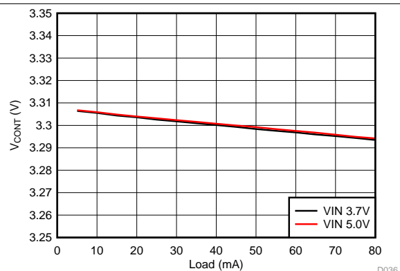
Figure 35. V CONT Load Regulation
