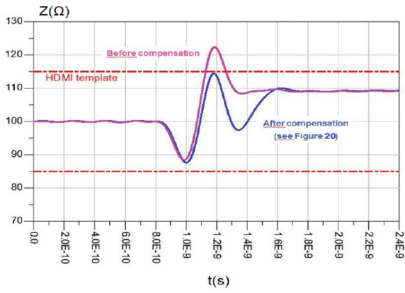
Figure 14. TDR
