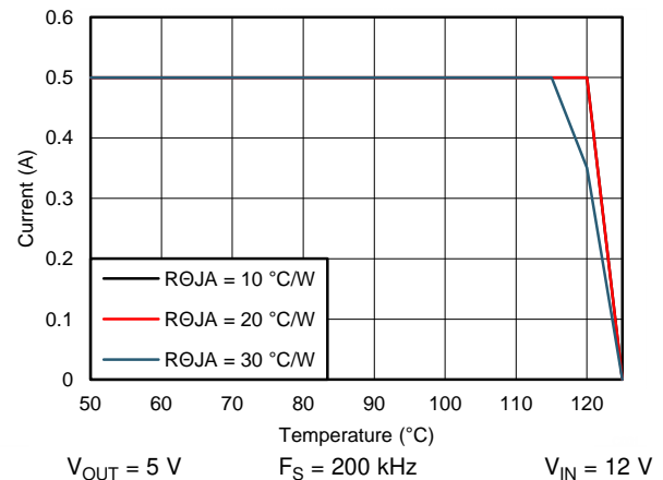
Figure 70. Derating Curve
